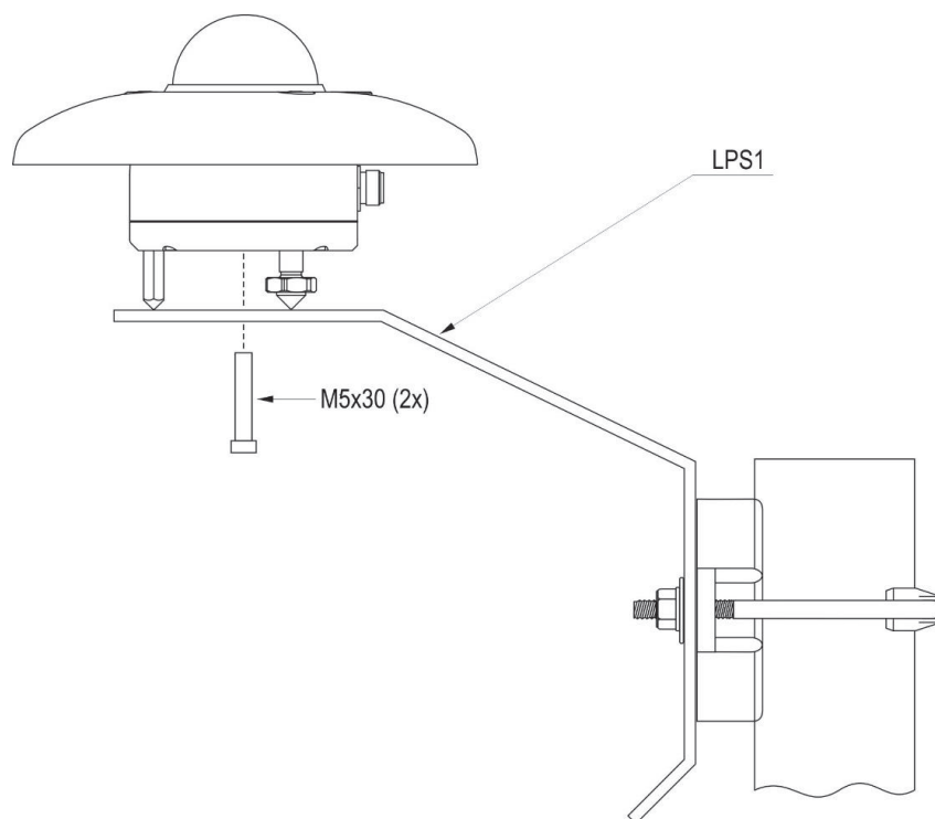
Fig. 4.2: LPS1 bracket for mast
