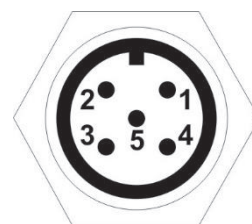
Pyranometer male connector
