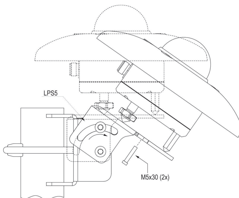
Fig. 4.3: LPS5 adjustable bracket for mast
